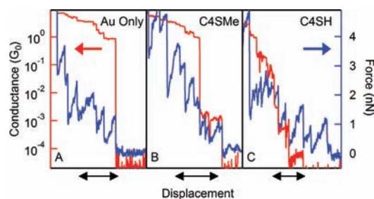
Figure 1. Sample conductance (red) and force (blue) traces for Au only (A), C4SMe (B), and C4SH (C). Arrow indicates a 0.5 nm displacement.
